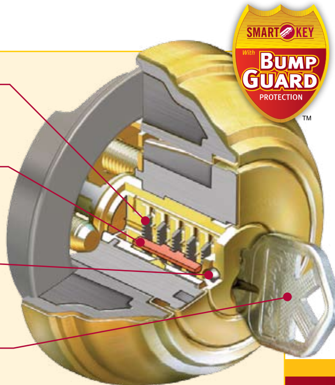
* 980 Deadbolt
